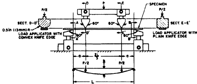
(Test Method C) FIG. 4 Four-Point Bend Test
