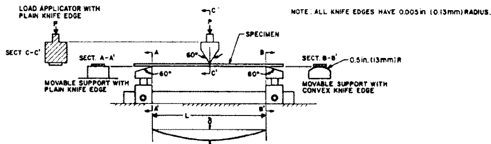
FIG. 3 Three-Point Bend Test
